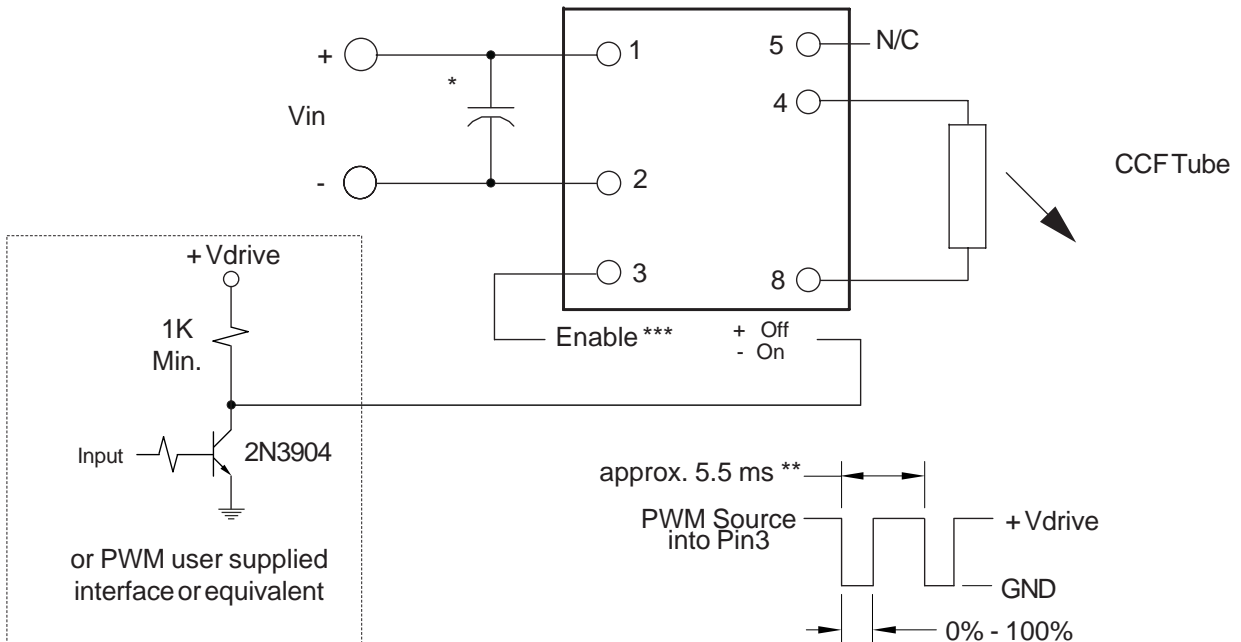
Figure 1: Connection Diagram
