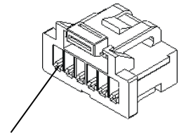
Pin 1 Molex 501330-0600 "CONN 1"
