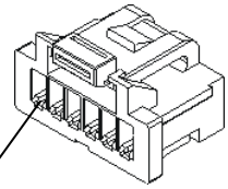
Pin 1 Molex 501330-0600 "CONN 2"
