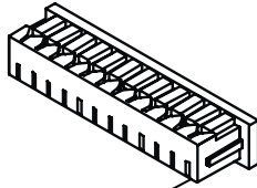
Pin 1 Molex 51021-1200 "CONN 1"
