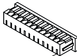
Pin 1 Molex 51021-1200 "CONN 1"
