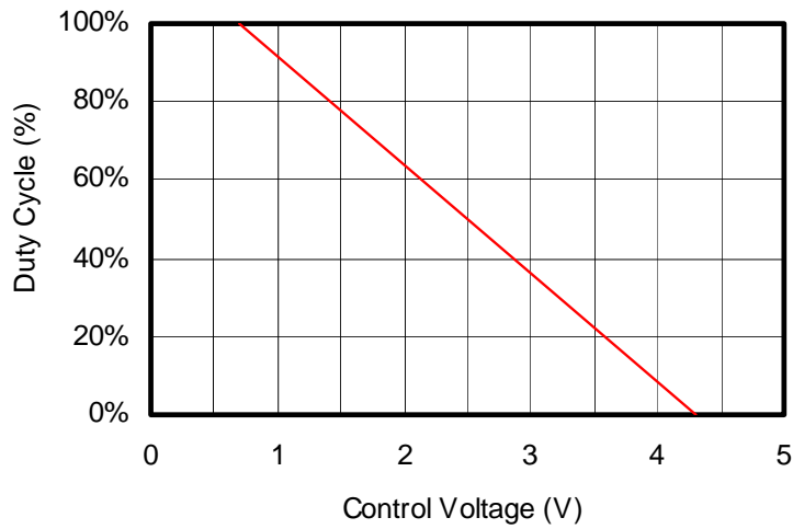
Control Voltage vs. Duty Cycle
