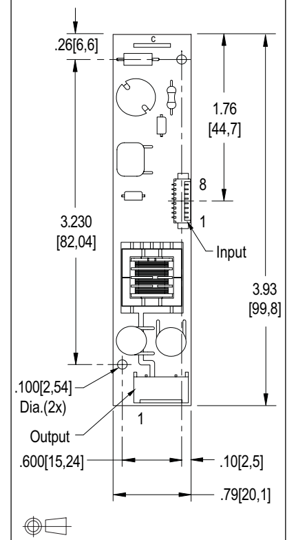
8mA Package
